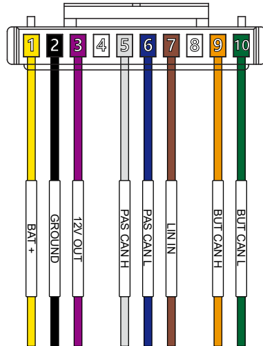
POWER/CAN CABLE
