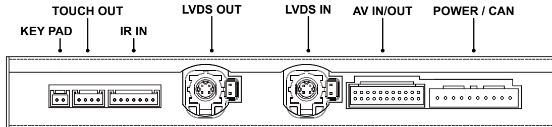
POWER/CAN CABLE
