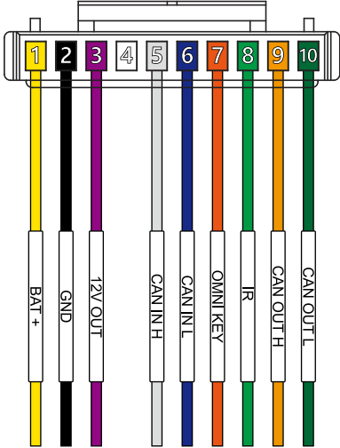
POWER / CAN CABLE
