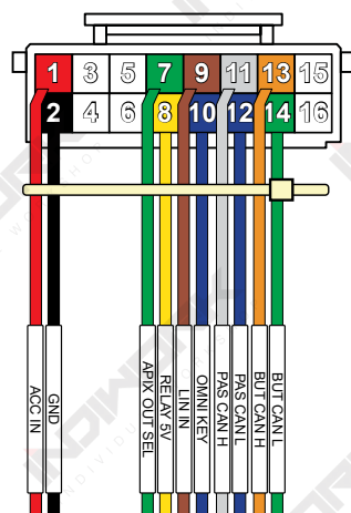
POWER/CAN CABLE
