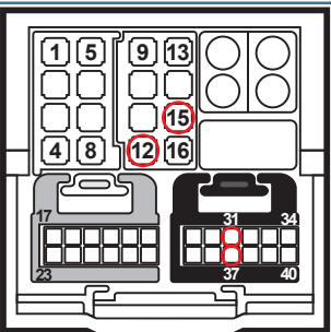
Original Main-Harness
